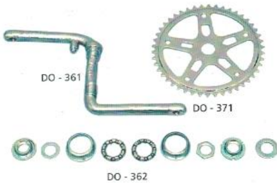
DO - 361 ONE PIECE CRANK Made of Special forged carbon steel BCP Size = 4-1/2" / 5-1/2" Thread = 1/2" x 20 TPI
